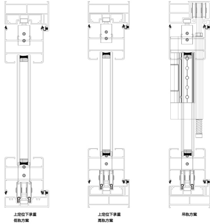
五金配件 Hardware fittings
